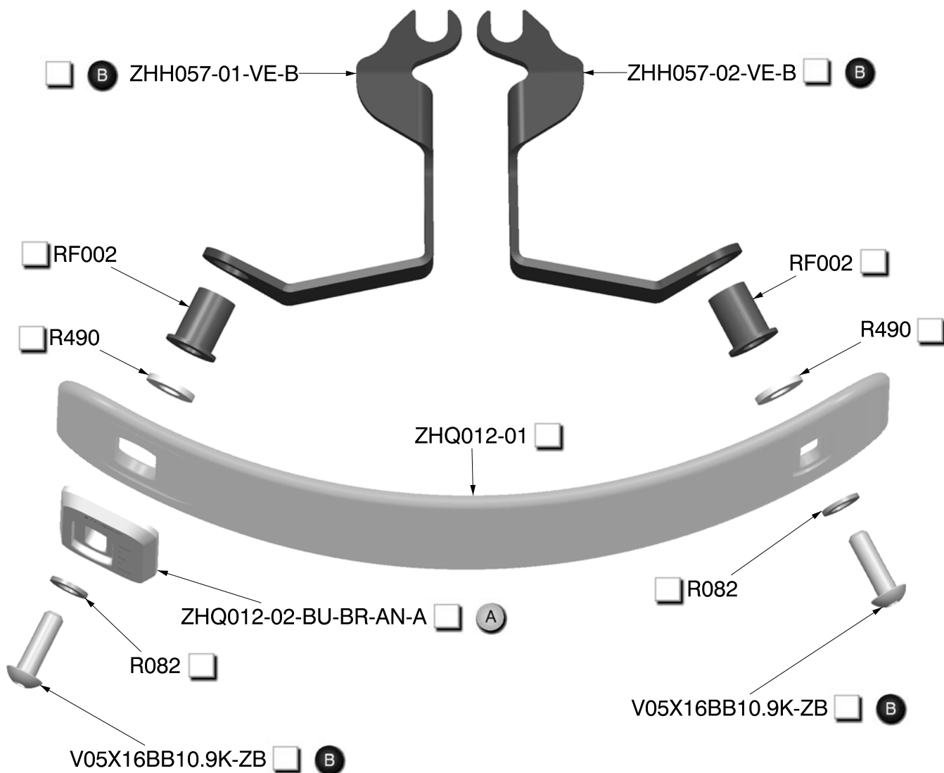
ZHH057 (Cupolino completo) (Complete headlight fairing)
