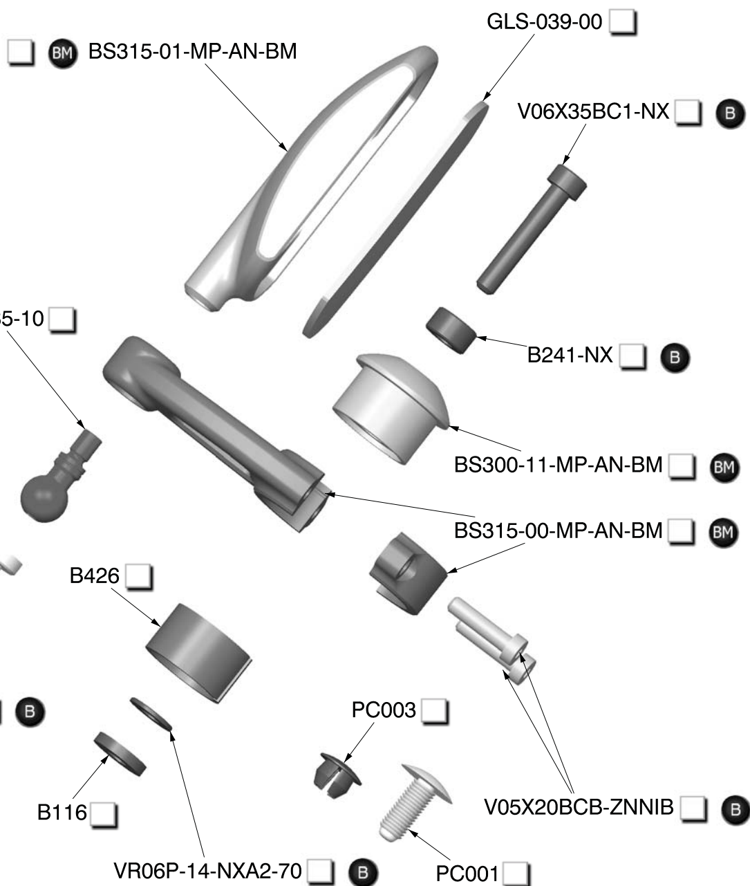
BS315 (Specchietto completo) BM (Complete mirror)
